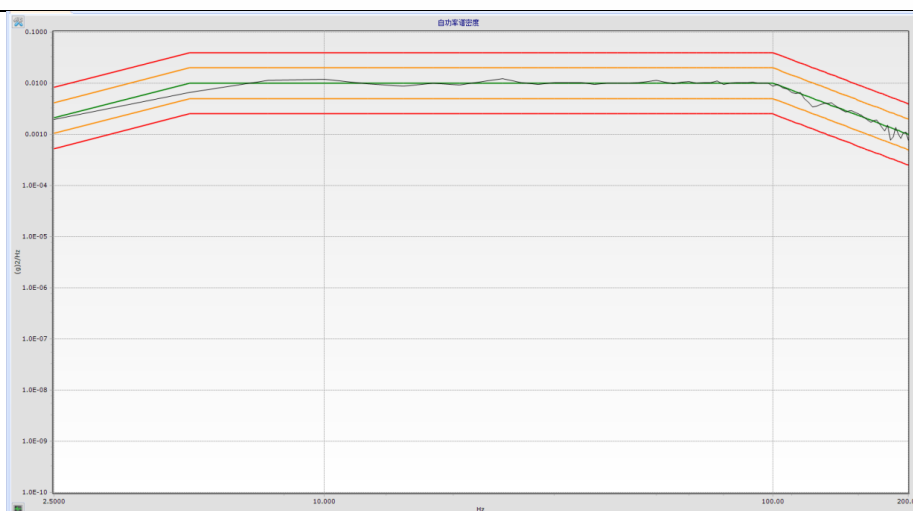
Test curve of Vibration (face 1)
